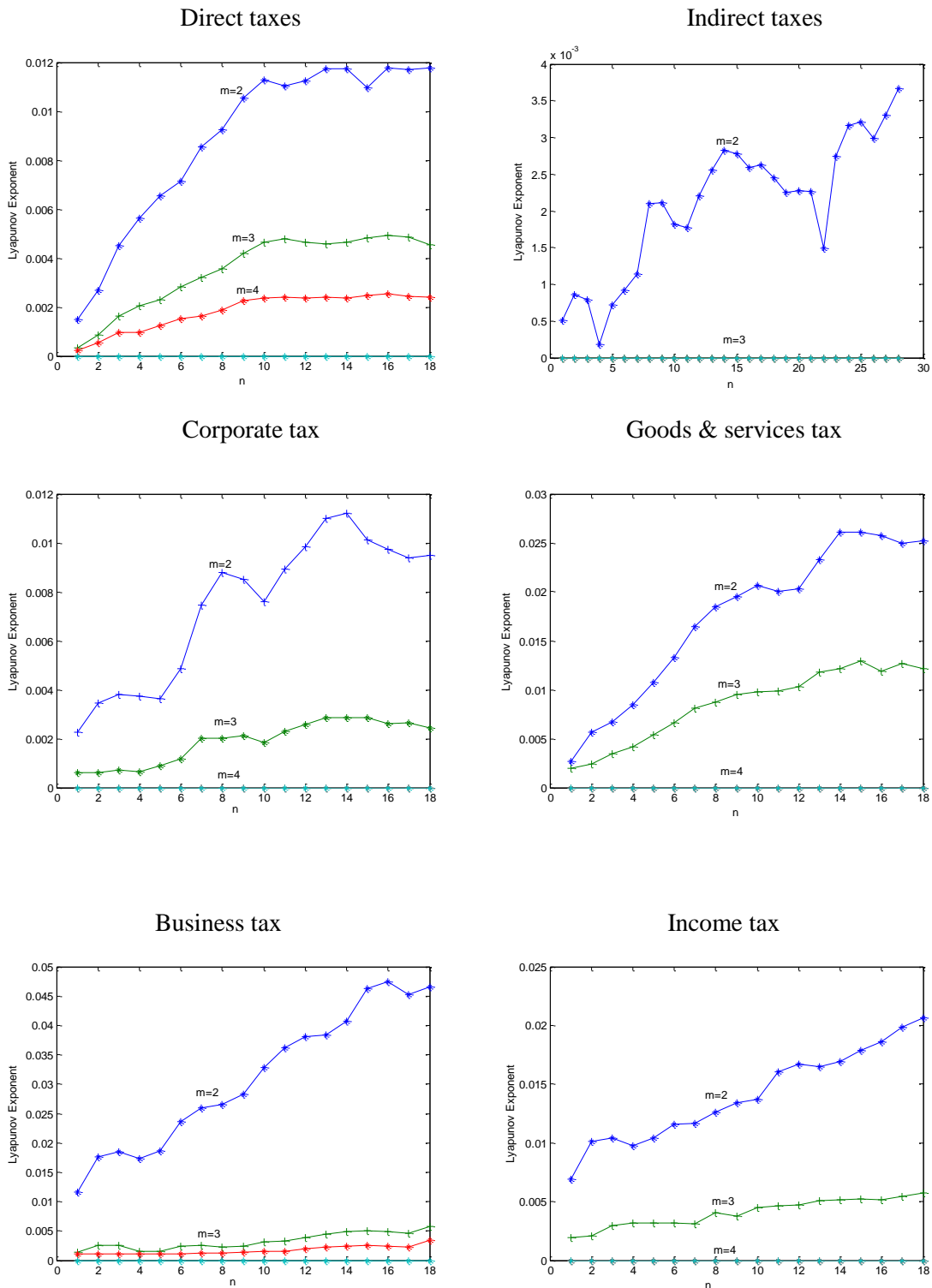
Figure 1. Lyapunov Exponent of taxes time series in different dimensions
